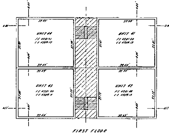
BUILDING "A"
